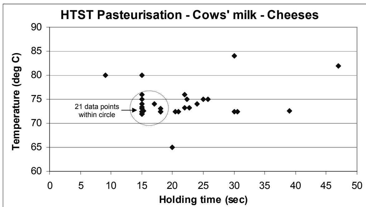
Figure 3.2. Temperatures and times of holding used by Australian dairy manufacturers for the HTST pasteurisation of raw cows’ milk used for the manufacture of all types of cheese. N = 48.
